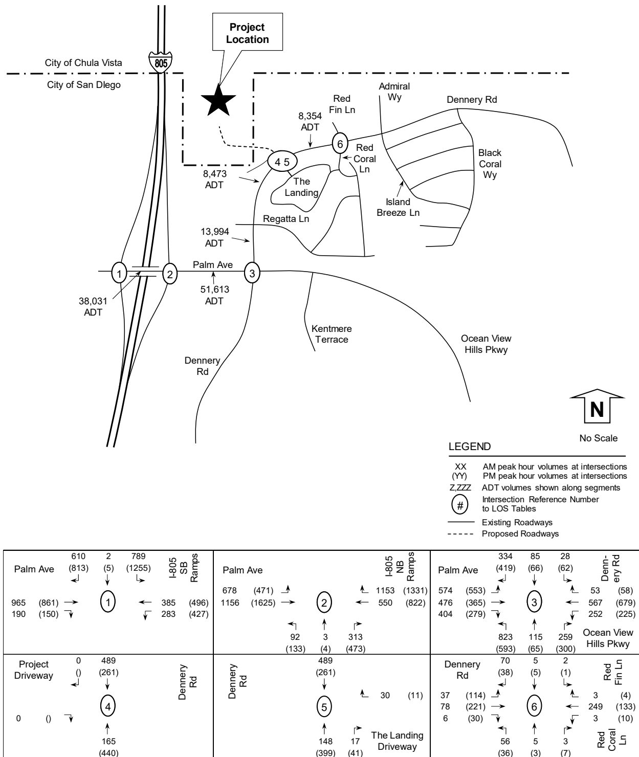
Figure 11: Opening Year 2025 without Project Volumes
