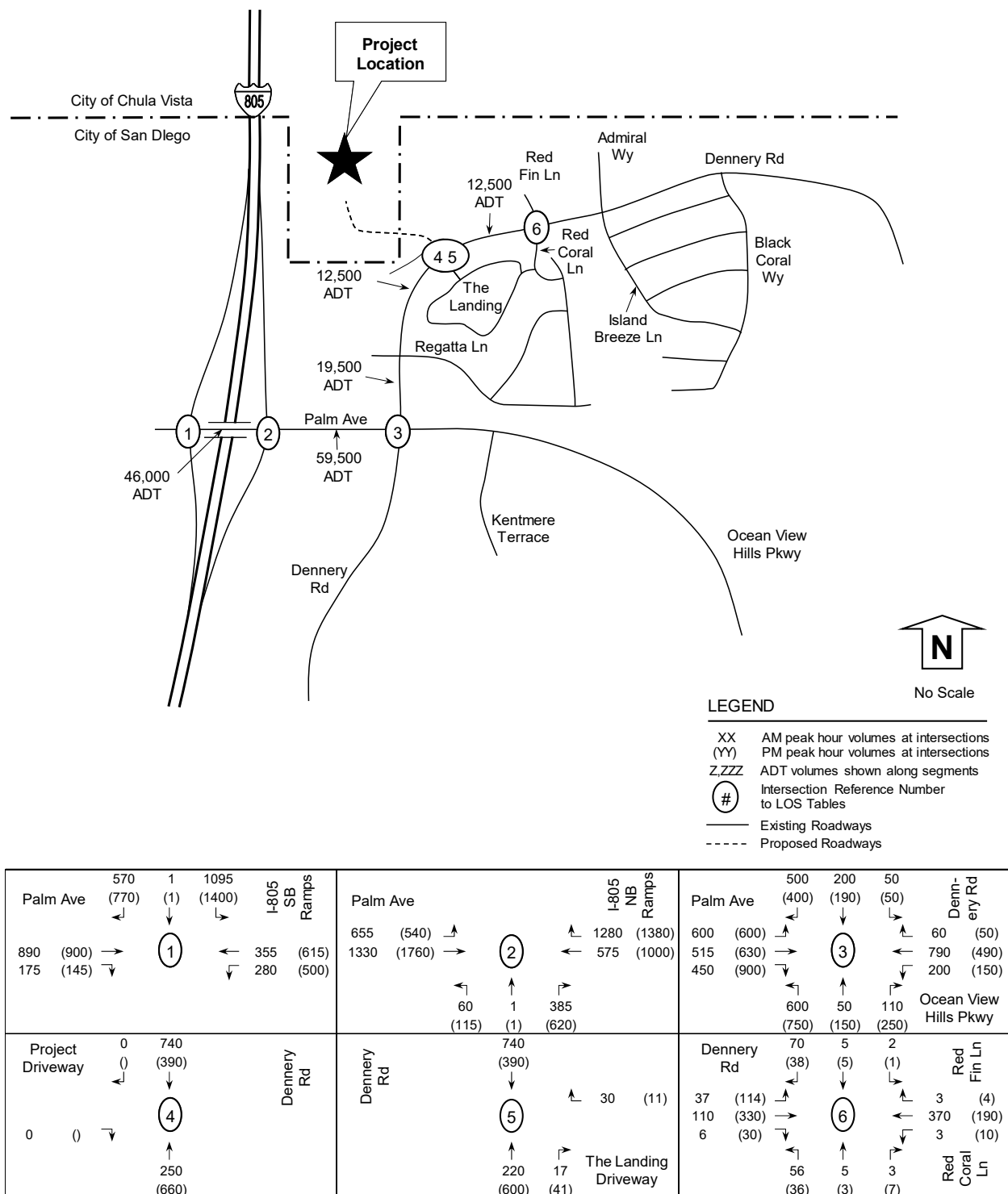
Figure 14: Horizon Year 2062 without Project Volumes
